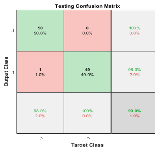
Figure 6. Testing Confusion matrix
